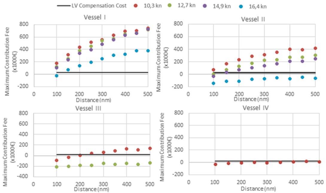
Fig. 6. Maximum contribution fee for vessel under base case conditions.
