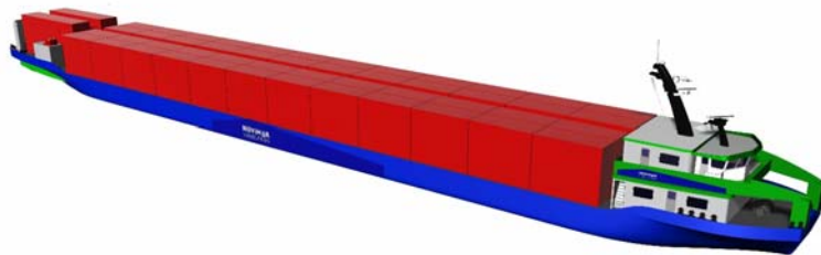
NOVIMAR Class Va, Shallow draft aft access Container ro-ro vessel
